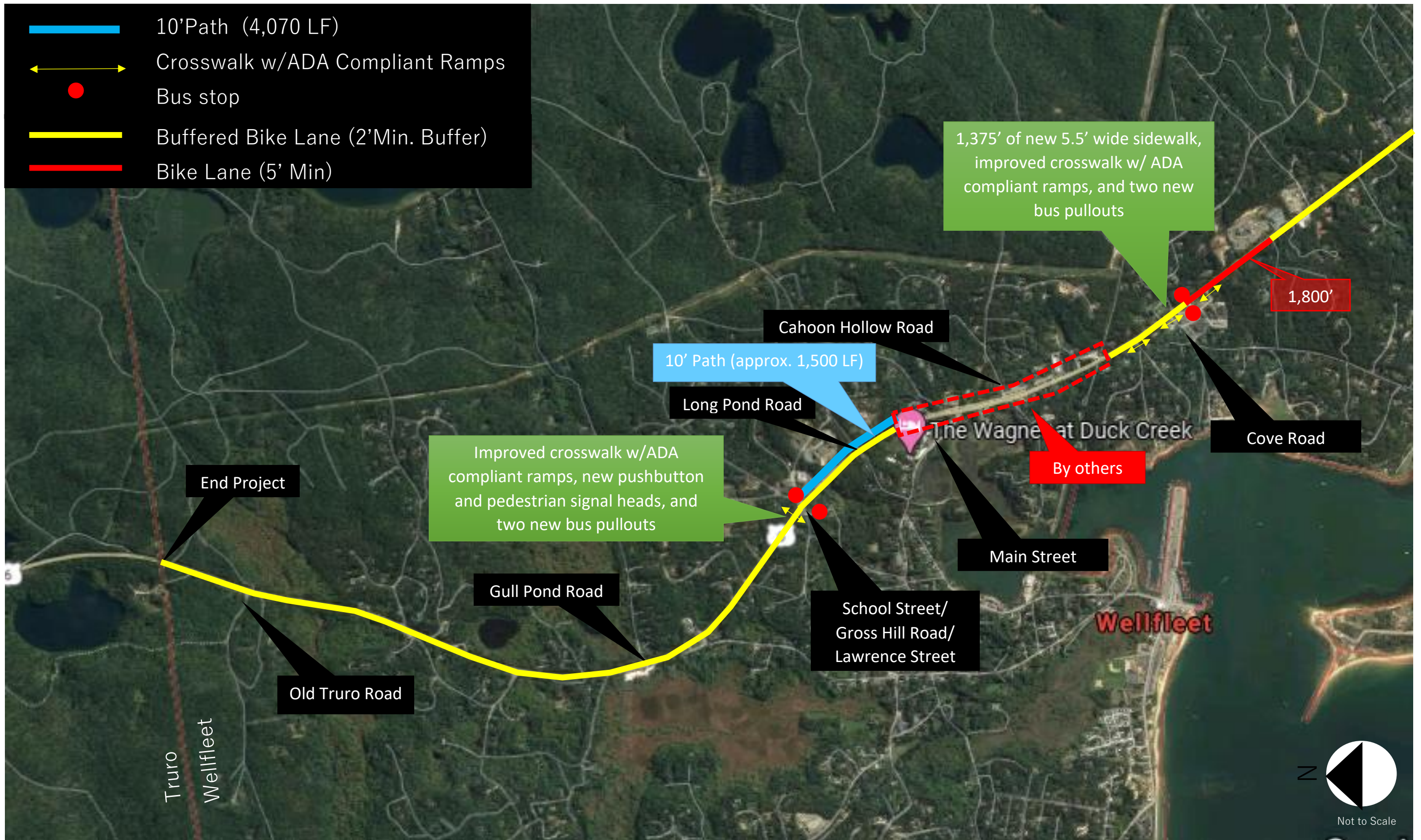
Route 6 – Wellfleet Pavement Preservation Project (MassDOT Project No. 609098) Proposed Pedestrian, Bicycle and Transit Improvements (Northern Portion of Corridor)
