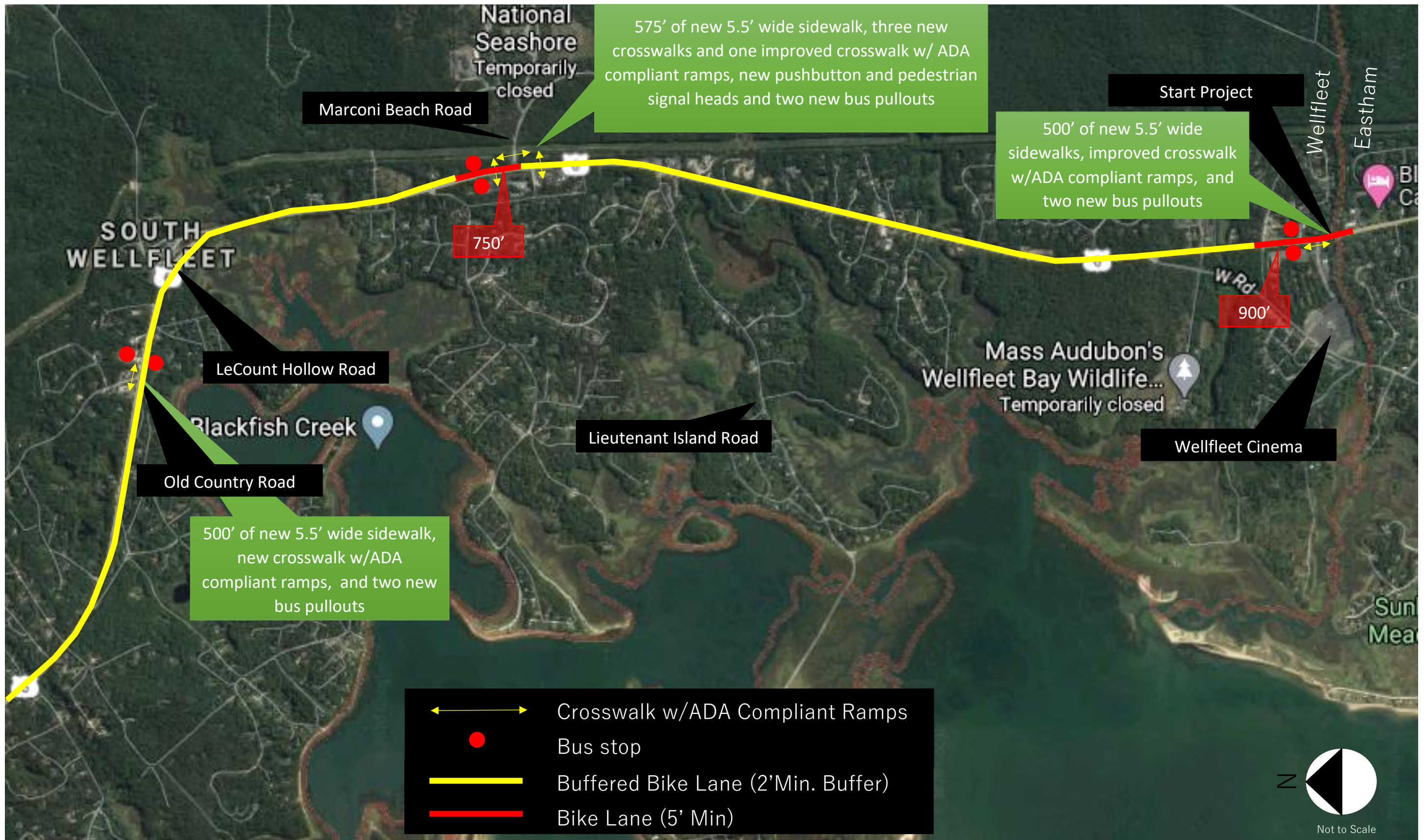
Route 6 – Wellfleet Pavement Preservation Project (MassDOT Project No. 609098) Proposed Pedestrian, Bicycle and Transit Improvements (Southern Portion of Corridor)
