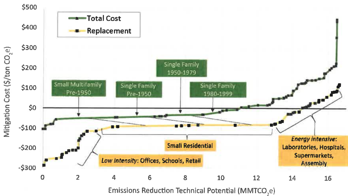
Figure 9. Emissions abatement cost curves based upon total or replacement capital costs of building electrification with only moderate efficiency to existing and new buildings. Each segment represents a building typology defined by use (e.g., office) and vintage (e.g., Pre-1950). Analysis assumes a 3% discount rate, and a 30-year lifetime period. Ordering of building typologies changes are due to different costs assumptions used across the building stock: electrifying offices, schools, and retail often can have lower upfront costs than replacement of fossil fuel equipment.
