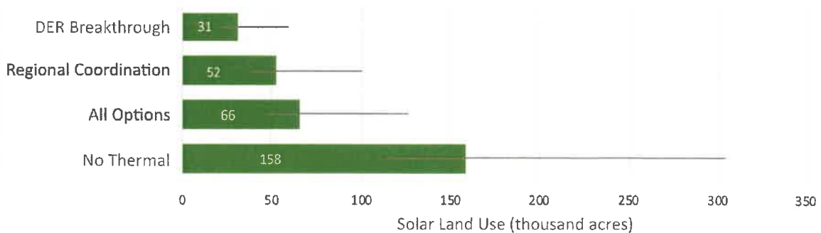
Figure 18. Ground-mounted solar PV land use estimates across pathways. Error bars show high and low land use estimates based on project design and technology progression. Fifty thousand acres represents approximately 1% of Commonwealth land area. Refer to Table 1 for a description of pathways.
