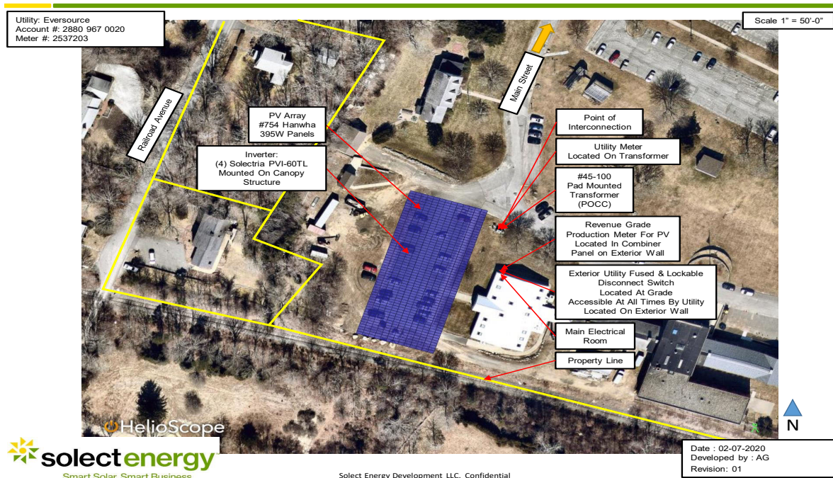
Site Plan – SED – Barnstable County Lab – 6177 – 320.45 kW DC – 240 kW AC 3195 Main St, Barnstable, MA 02630
